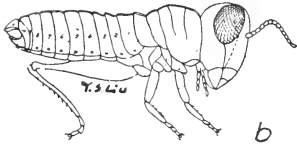
Fig. 51. a, Adelphocoris rapidus (Say); b, Melanoplus differentialis (Thomas).
